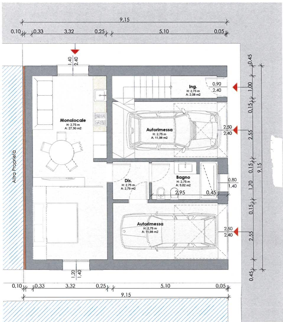
Piano Terra
